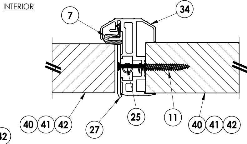
6 HORIZONTAL CROSS SECTION 5 Outswing shown (Inswing similar)
