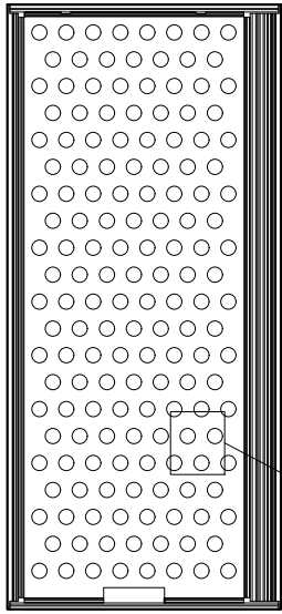
DOOR PANEL SECTION PANEL REINFORCEMENT (0.023" Thick Steel) STEEL REINFORCEMENT 28.86% OPEN AREA MAX.
